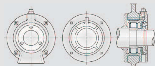
Fig. 26: Grease valve (plumber block)
