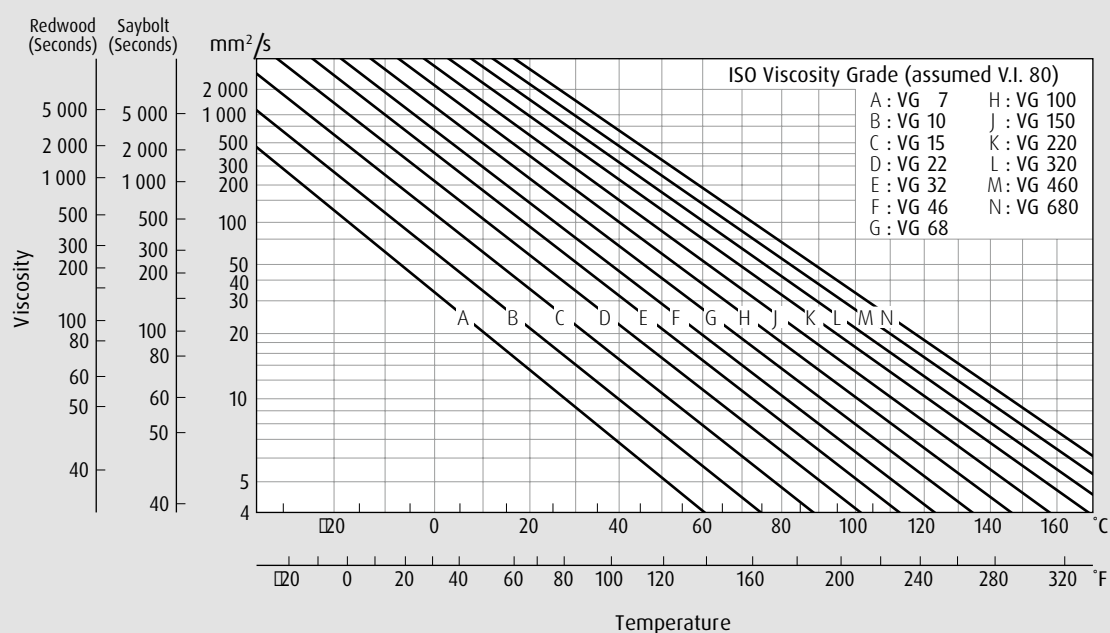
Fig. 21: Temperature-Viscosity chart
