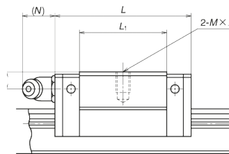
SIDE VIEW OF CL TYPE
