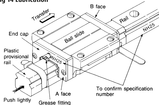
Fig 14 Lubrication
