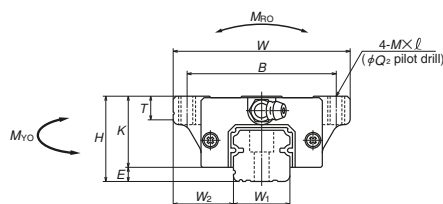
FRONT VIEW OF EM AND GM TYPES
