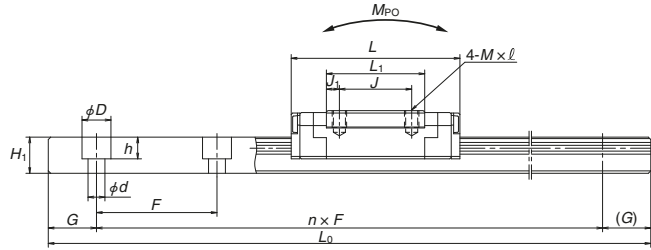
SIDE VIEW OF PU TYPE
