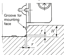
Fig 9 Rail Datum Face Mounting Part
