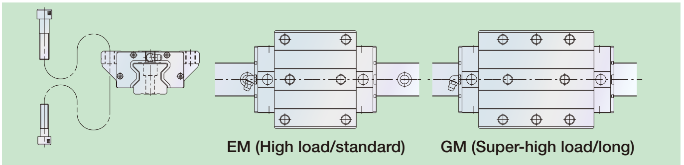
Fig. 5 Flanged type
