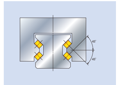
Balanced four-directional equal load specification
