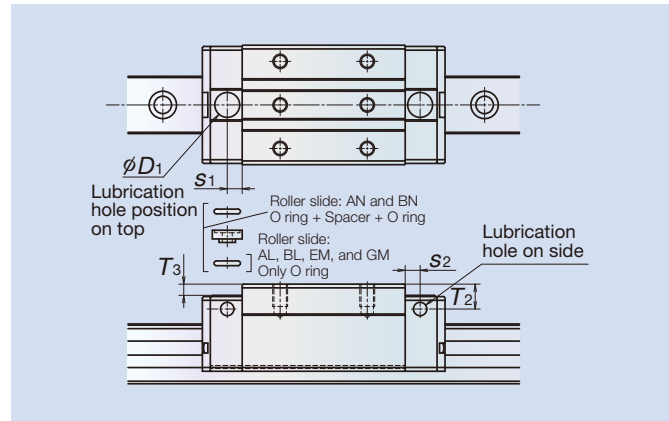
Fig. 11 Top and side lubrication hole positions
