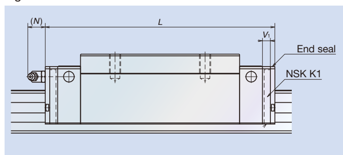
Fig. 15 Slide with NSK K1
