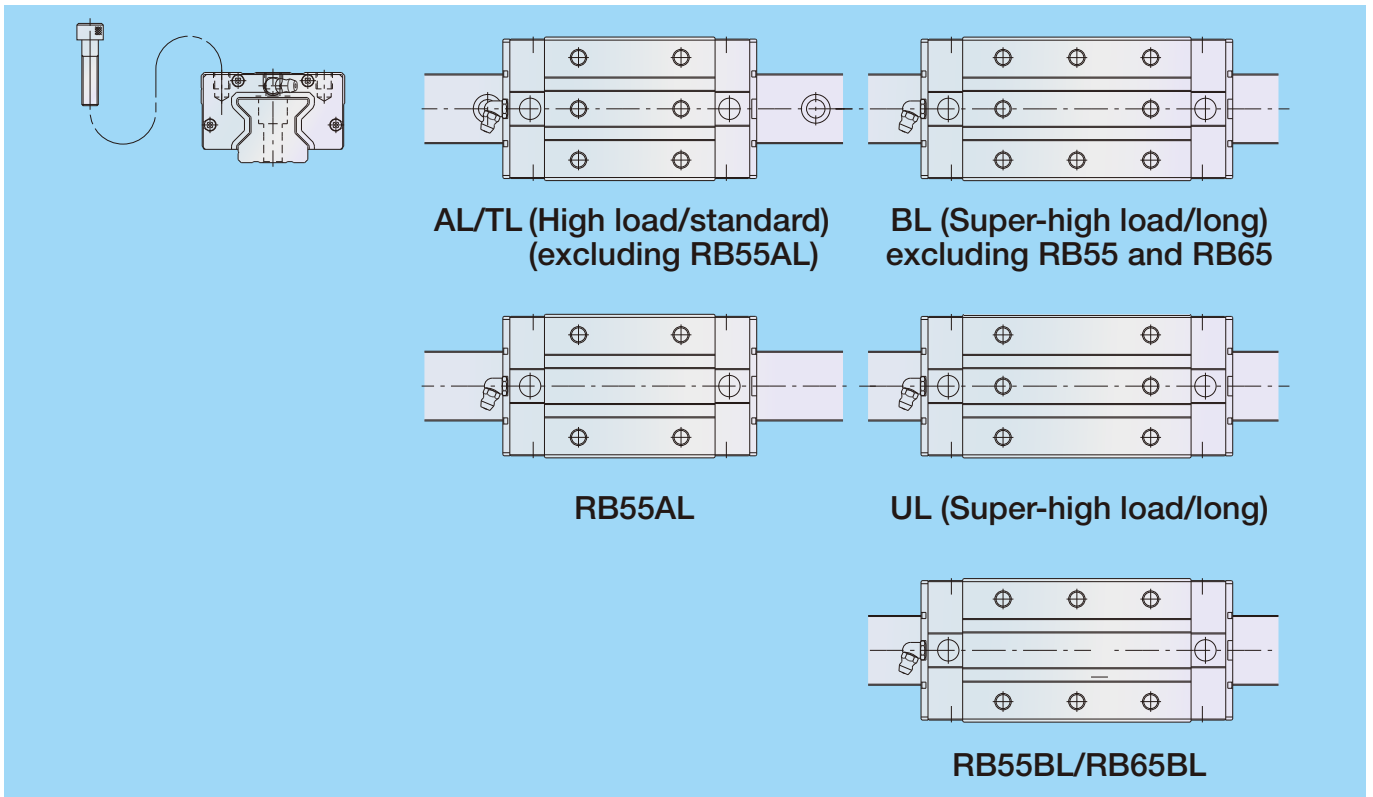
Fig. 4 Low-profile type
