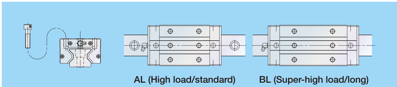
Fig. 2 Low-profile type
