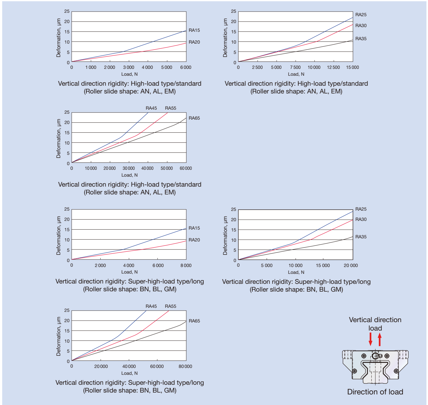
Fig. 7 RA model: Theoretical vertical direction rigidity
