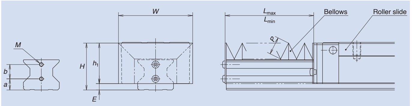
Fig. 18 Bellows dimensions
