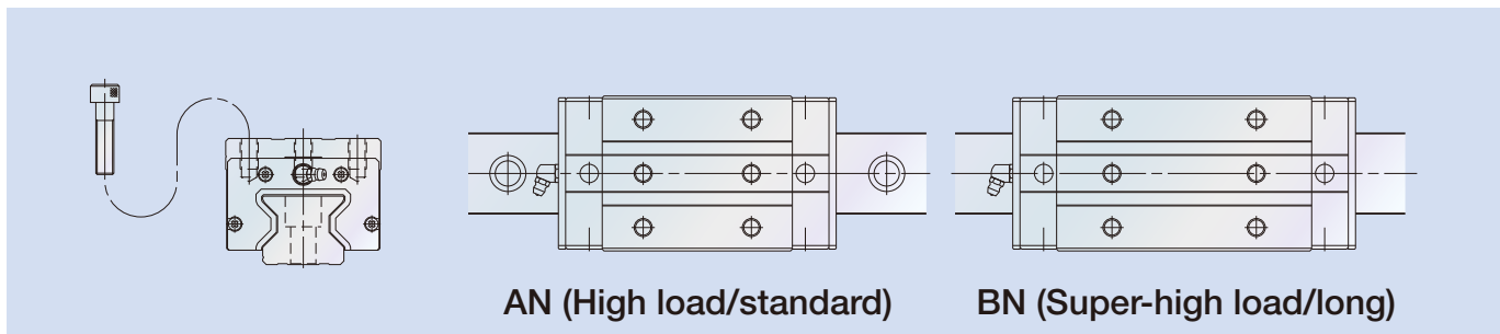
Fig. 1 Square type
