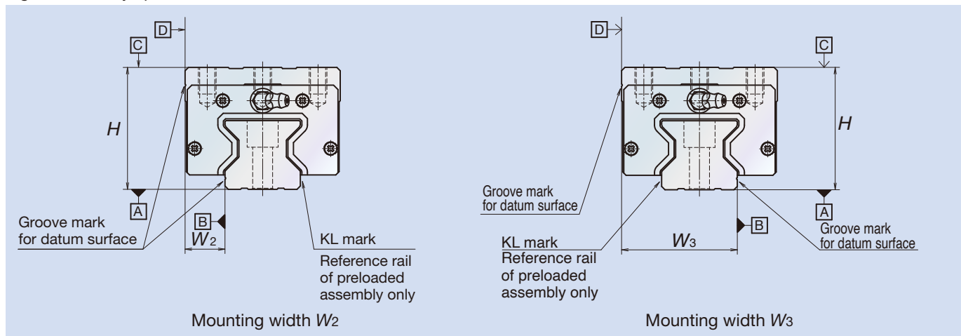
Fig. 6 Accuracy specifications
