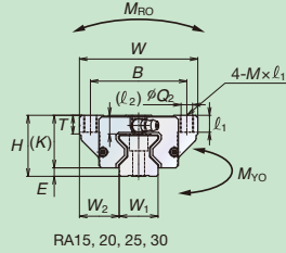
Front view of EM and GM types
