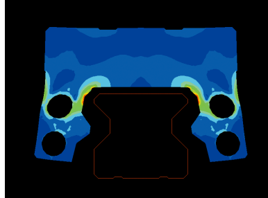
Example roller slide deformation analysis
