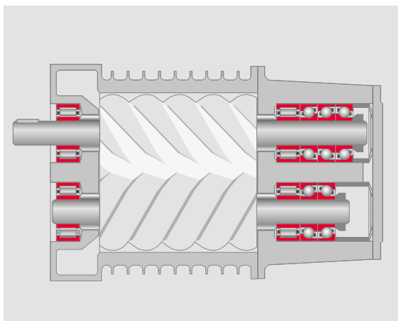
High load capacity Cylindrical Roller Bearings with L-PPS cage
