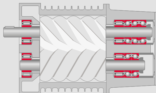
Typical Refrigerant – Screw Compressor
