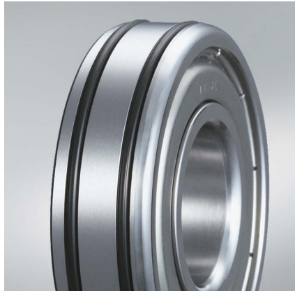
Creep-Free bearing
